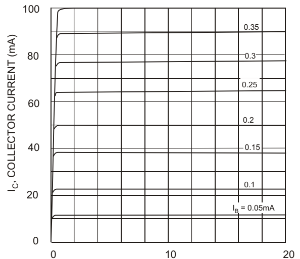
Fig. 6, Typical Emitter-Collector Characteristics
